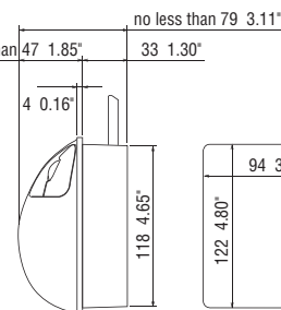
Cutout for flush mount
